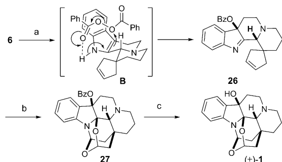
Scheme 6. Total synthesis of (±)-terengganensine A ( rac -1): a) Bz 2 O 2 (DBP), CHCl 3 , RT, 68%; b) OsO 4 (0.02 equiv), NMO, 2,6-lutidine, Me 2 CO–H 2 O, RT, then PIDA, RT, 76%; c) 1.0% NaOH, MeOH, 40°C, 95%.
